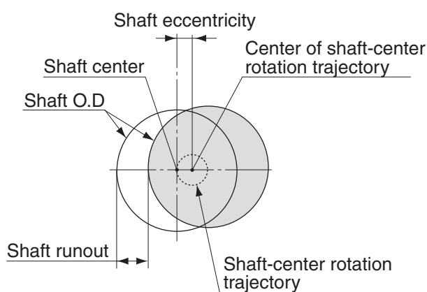
Fig. 1.5.5 Shaft runout
