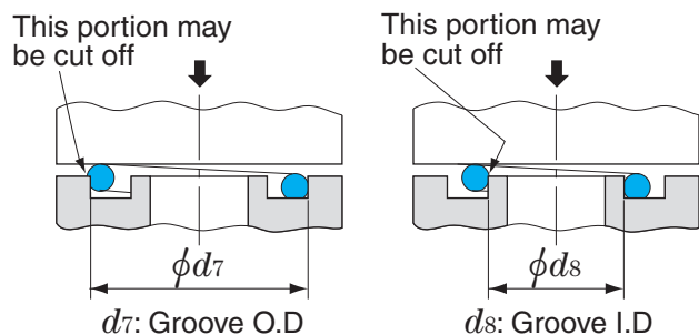
Fig. 2.4.5 O-ring protrusion
