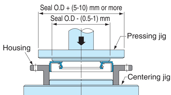
Fig. 1.7.3 Recommended seal press-fitting jigs
