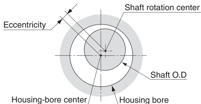
Fig. 1.5.6 Housing bore eccentricity
