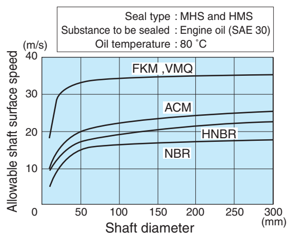
Fig. 1.6.3 Relation between rubber materials and allowable peripheral speed for seal
